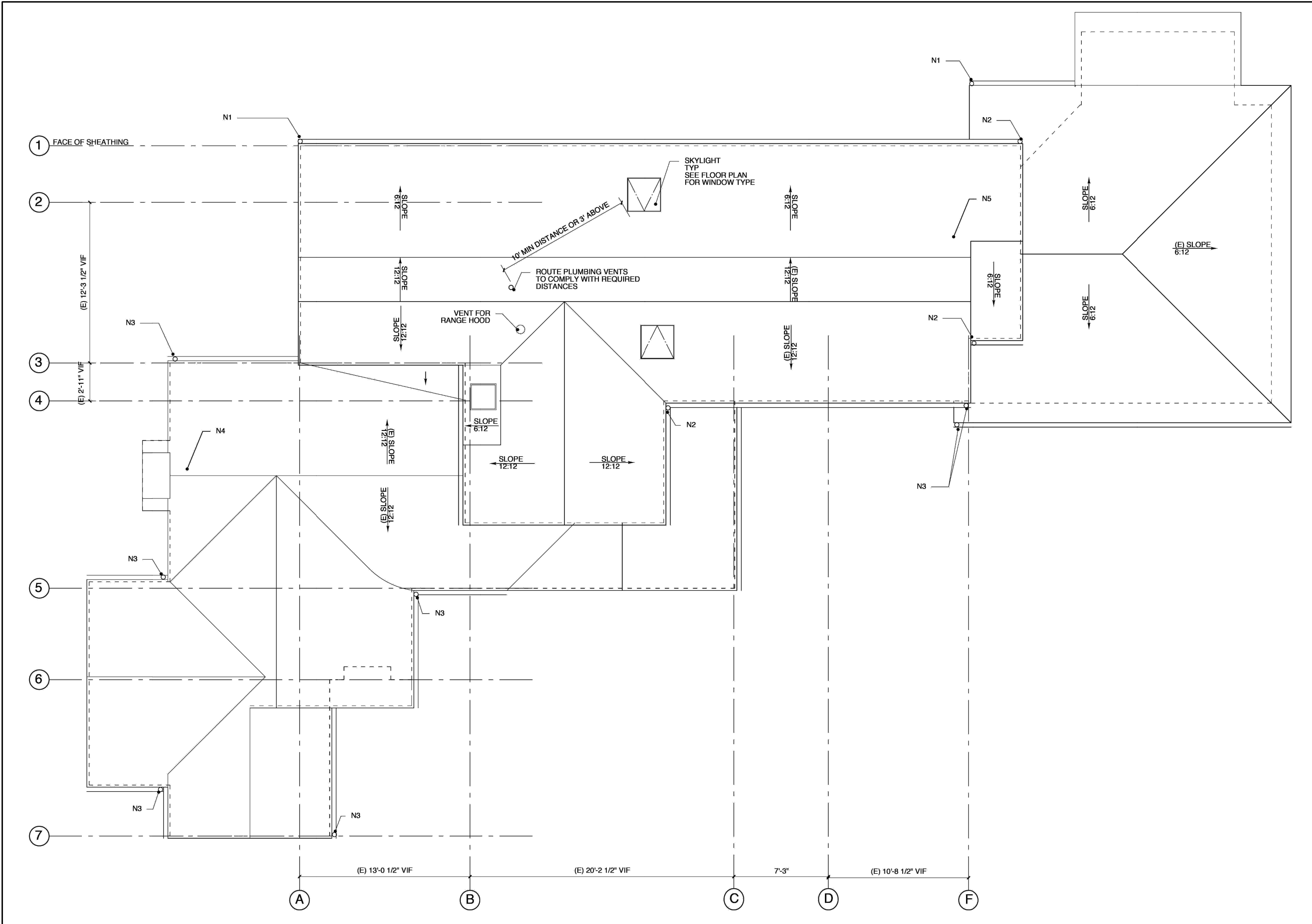
EXISTING ROOF PLAN 4
