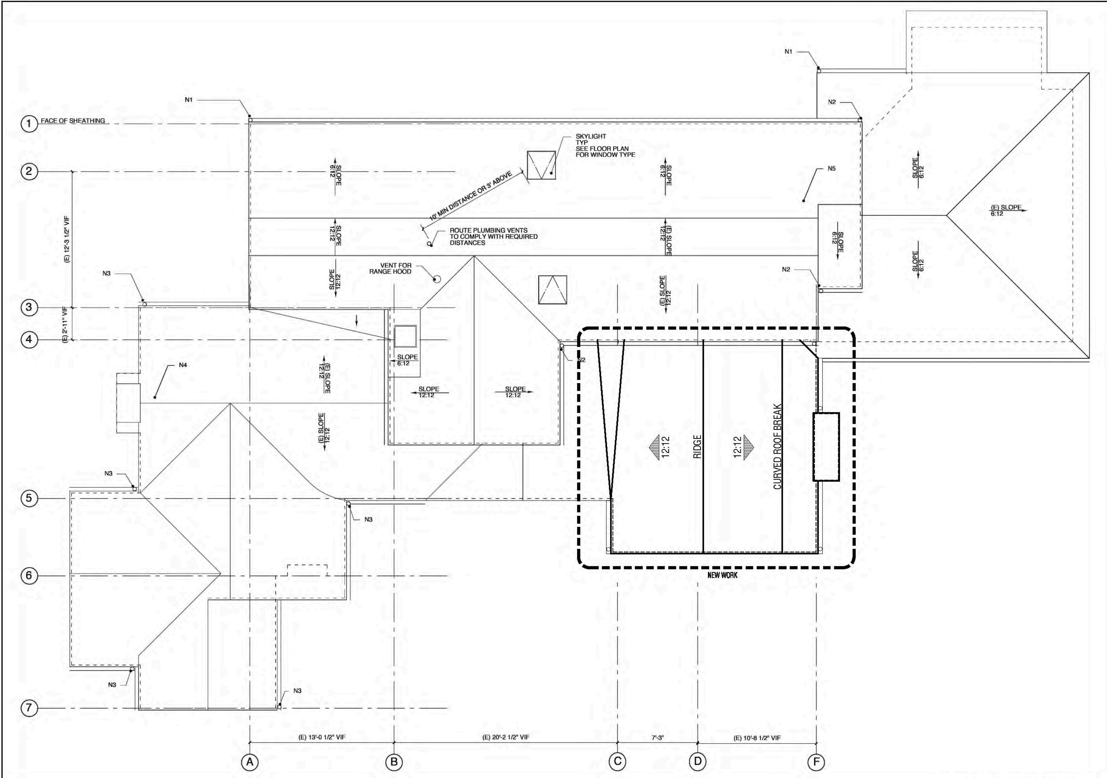
PROPOSED ROOF PLAN 4
