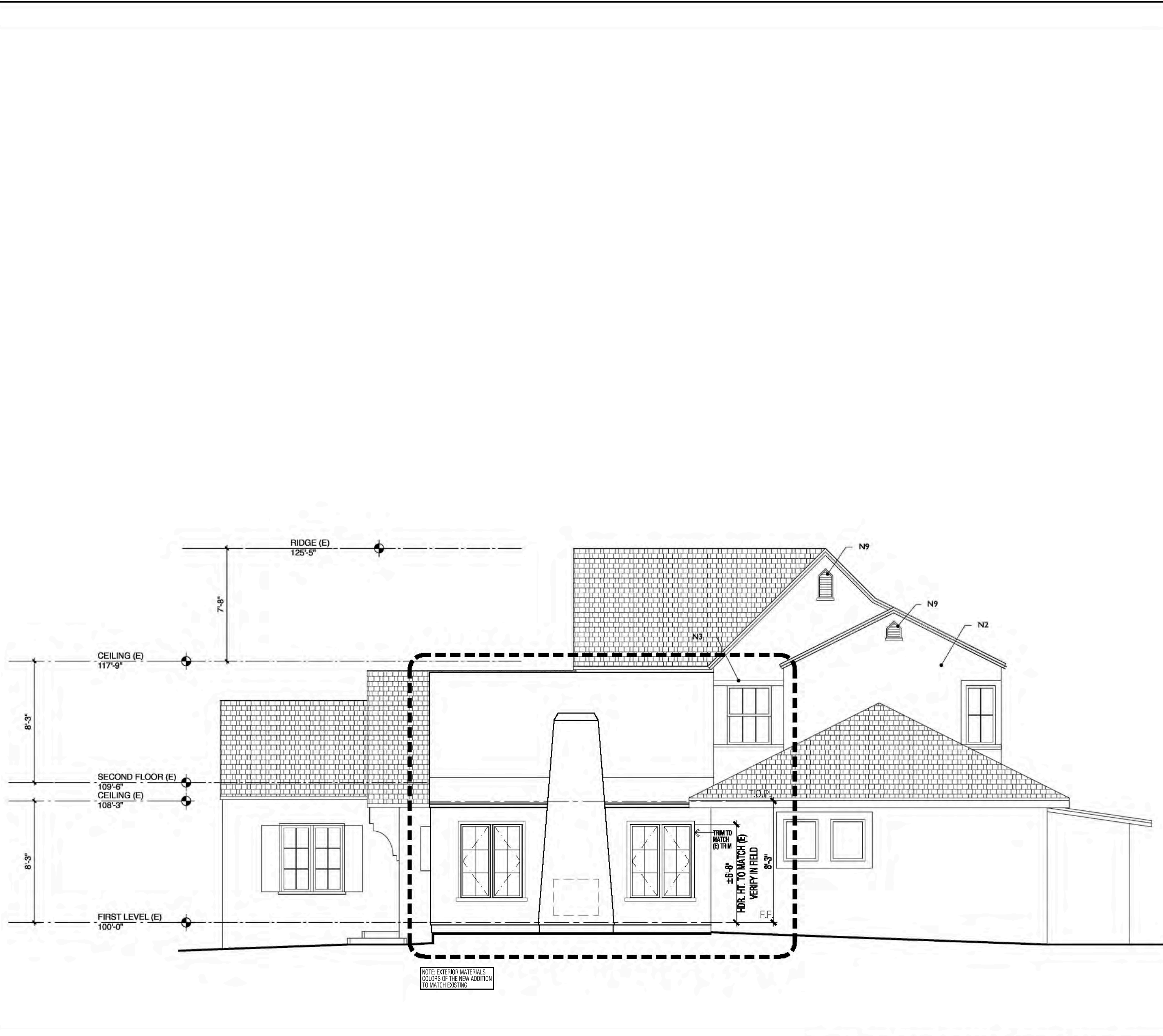
PROPOSED EXTERIOR ELEVATION : RIGHT 3
