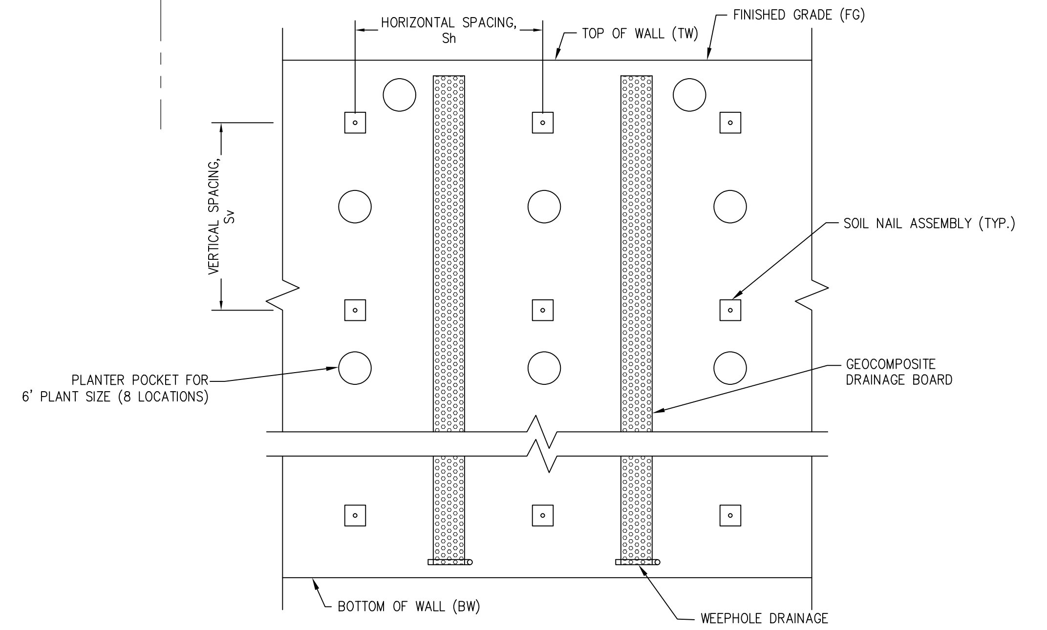
3 PARTIAL ELEVATION NO SCALE
